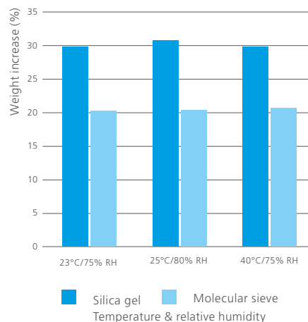
Moisture adsorption capacity of AdPack® after 24h for different climate conditions
