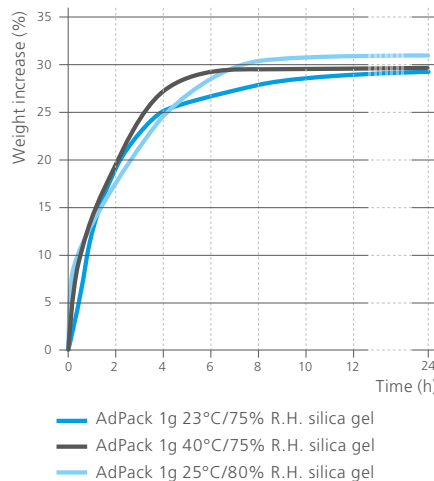
Moisture adsorption capacity of AdPack® 1g silica gel as a function of time at different conditions
