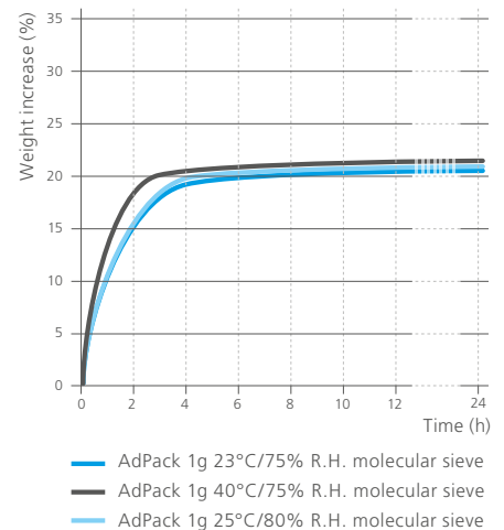
Moisture adsorption capacity of AdPack® 1g molecular sieve as a function of time at different conditions
